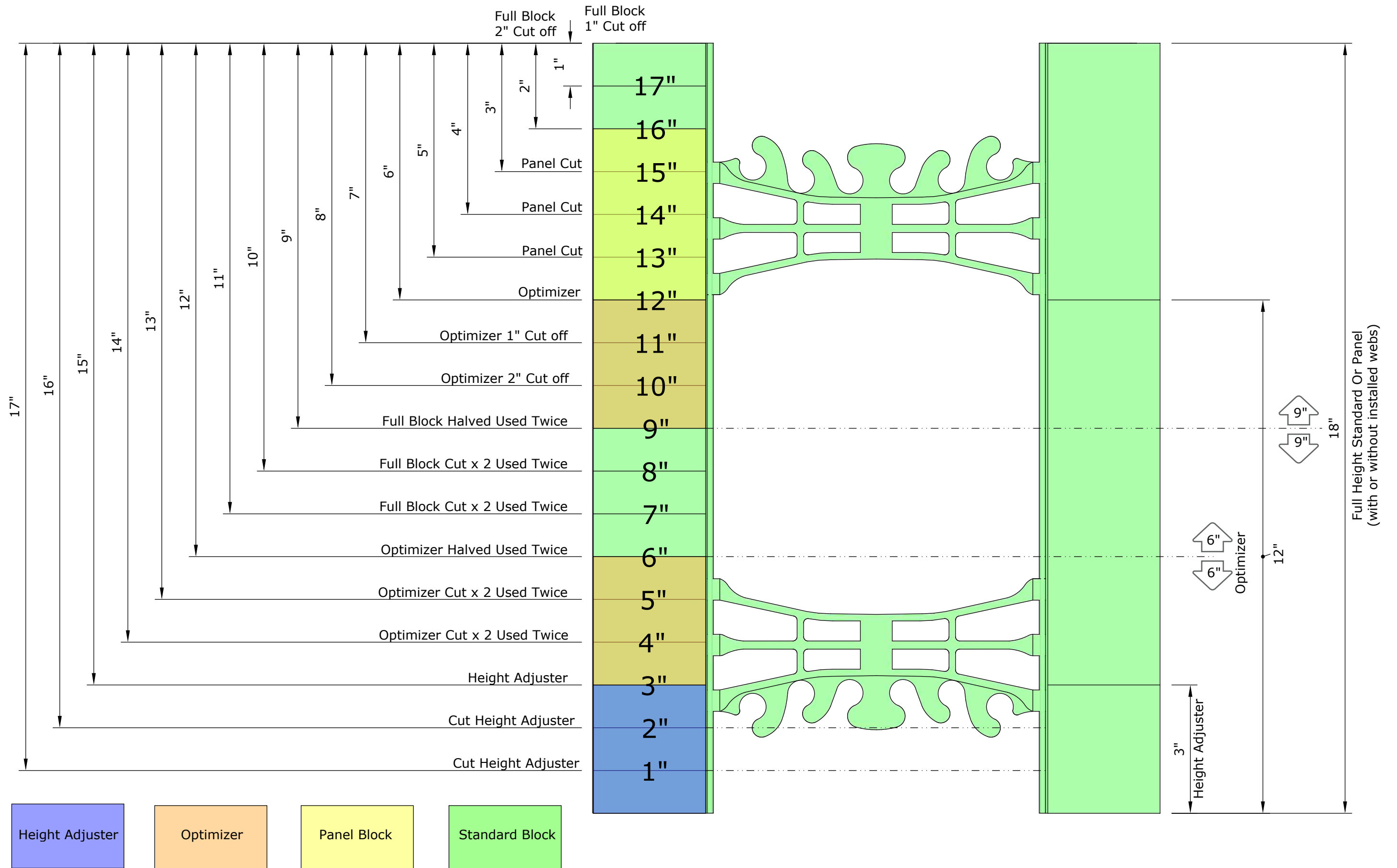
Drawing: Wall Height Composition Key
