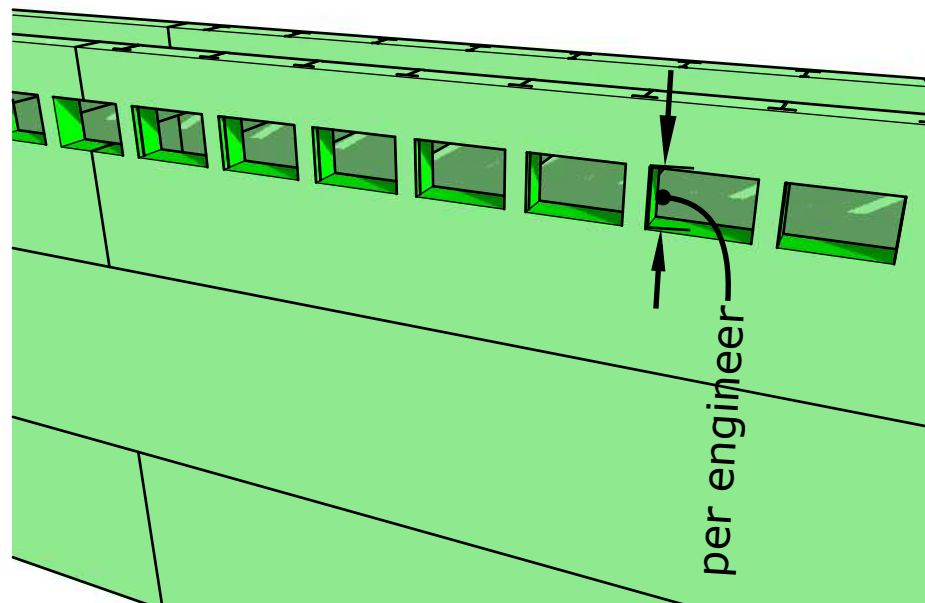
Cutouts Between ICF 8 inch Webs
