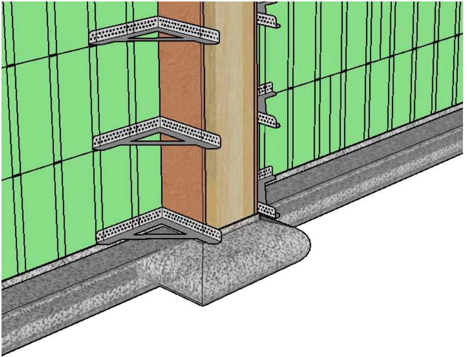
2 Pier Casing Screw Fixed To ICF Webs Ready For Pour
