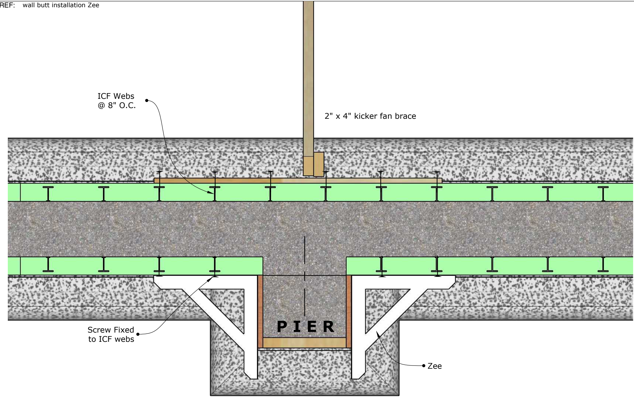
Plan View
